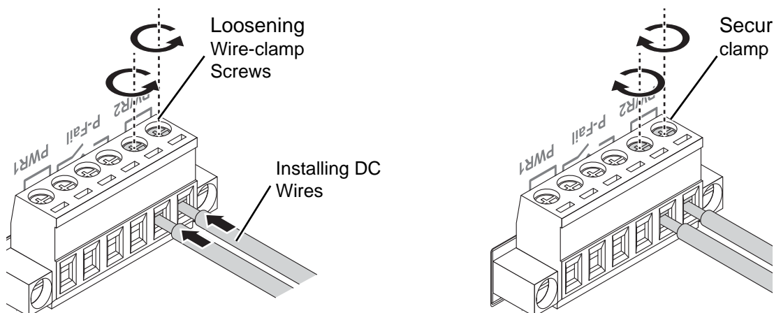
Figure 2.21 Installing DC Wires in a Terminal Block
