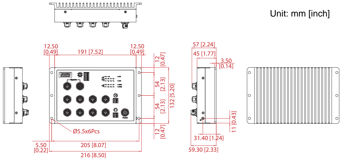
Figure 1.12 EKI-9510E-2GMPH/EKI-9510E-2GMPL Dimensions
