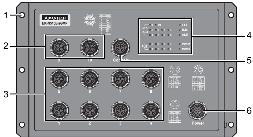
Figure 1.3 Front View
