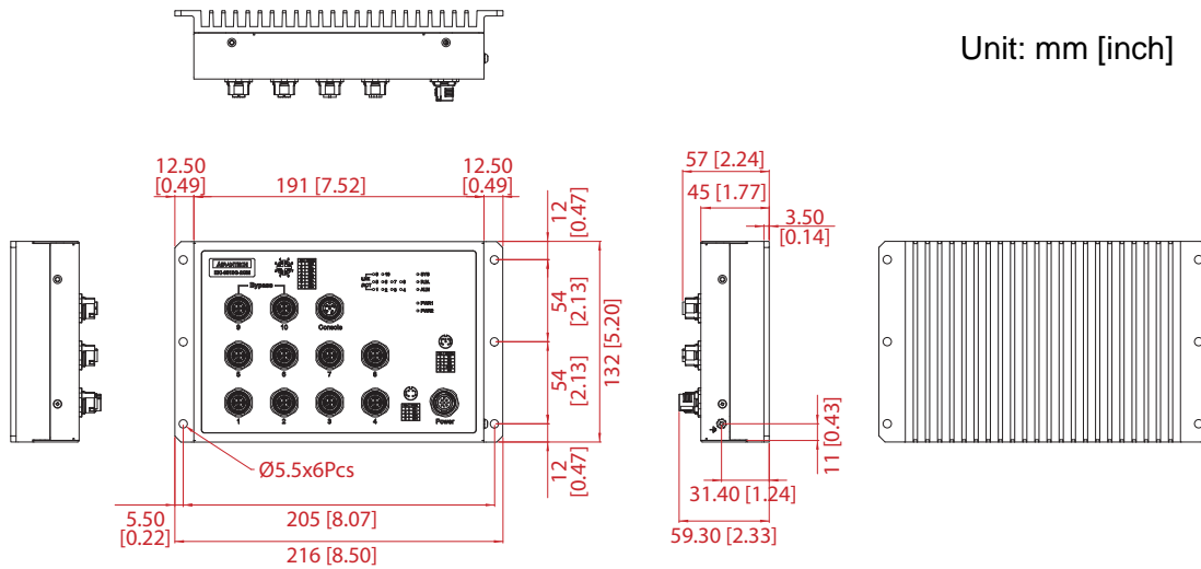
Figure 1.14 EKI-9510G-2GH/EKI-9510G-2GL Dimensions
