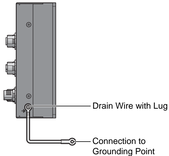
Figure 2.4 Grounding Connection, Chassis Left Side View
