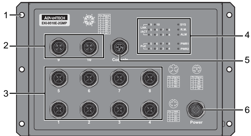
Figure 1.7 Front View
