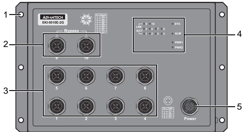
Figure 1.5 Front View
