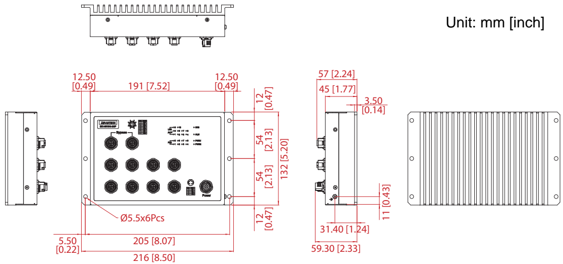
Figure 1.16 EKI-9510G-2GMPH/EKI-9510G-2GMPL Dimensions
