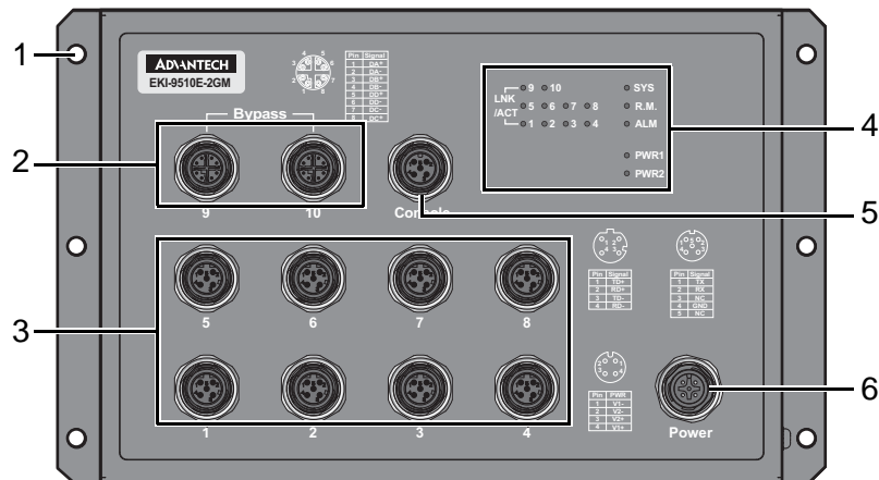
Figure 1.2 Front View
