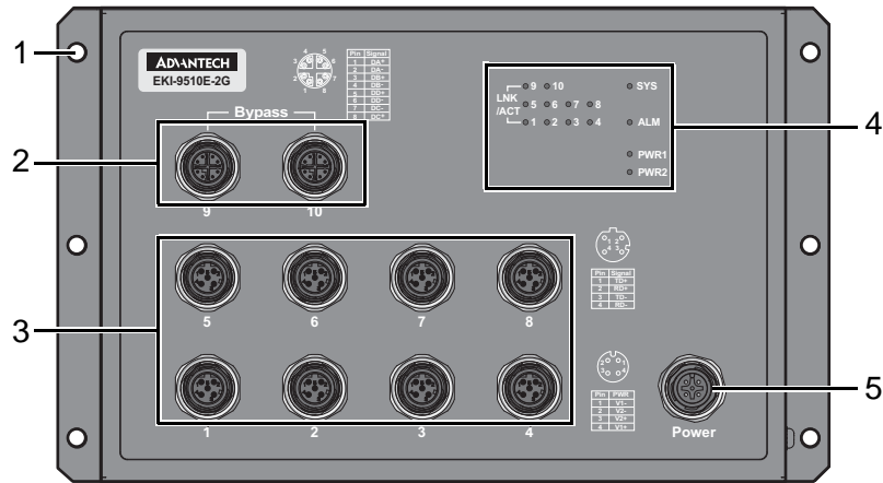
Figure 1.1 Front View
