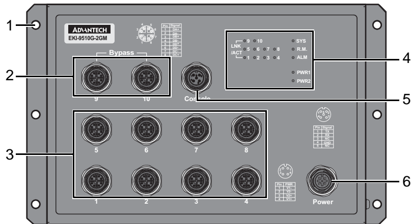
Figure 1.6 Front View
