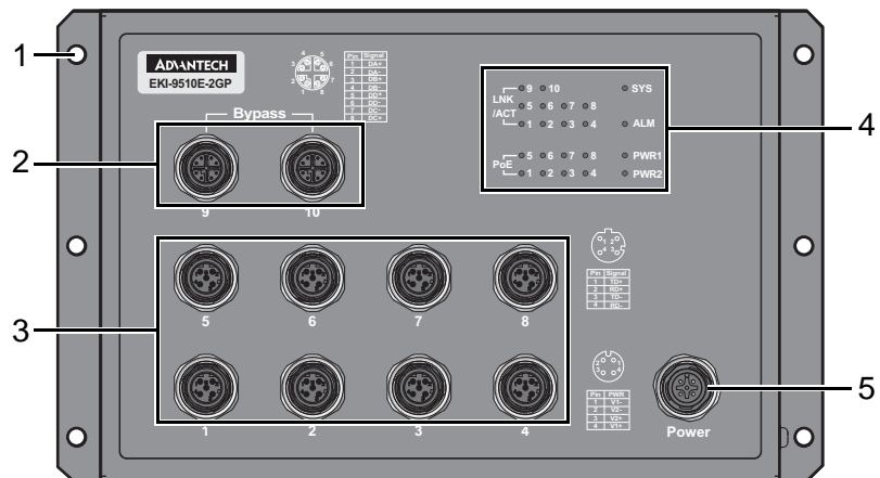
Figure 1.4 Front View
