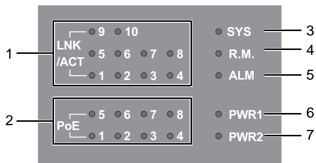
Figure 1.9 System LED Panel
