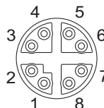
Figure 2.8 M12 X-Coded Connector Pin Assignment
