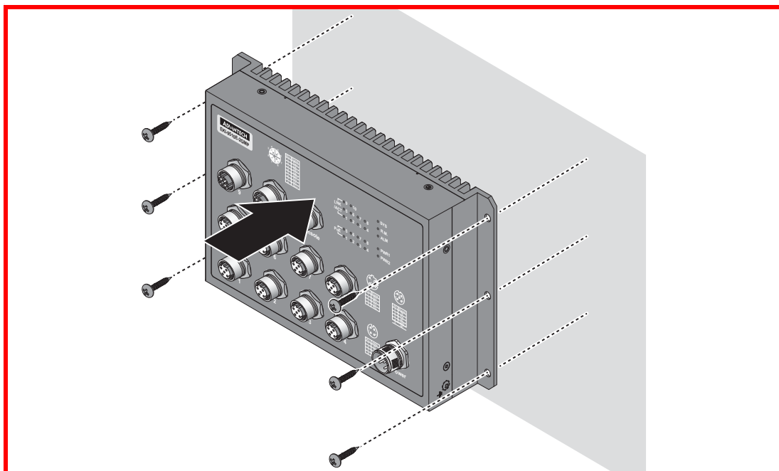
Figure 2.2 Switch Installation
