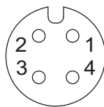
Figure 2.6 Standard M12 4-Pin Female DC Power Input Connector
