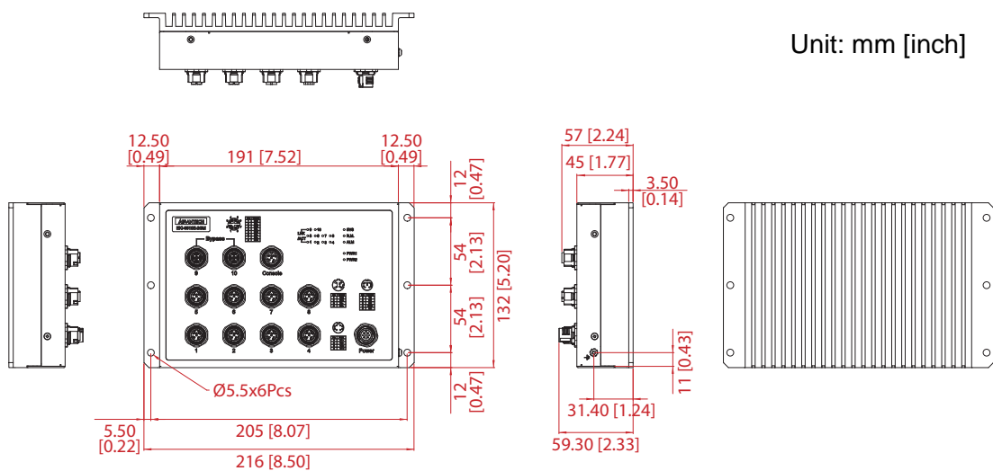
Figure 1.10 EKI-9510E-2GH/EKI-9510E-2GL Dimensions
