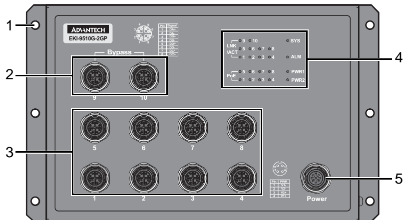
Figure 1.8 Front View
