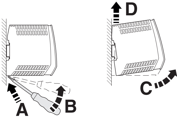
Figure 18 Removal
