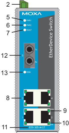
EDS-305-M-ST Front Panel View
