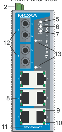
EDS-308-MM-ST Front Panel View
