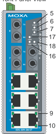
EDS-309-3M-ST Front Panel View
