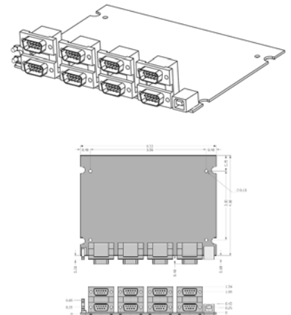
Board Layout for QSU Model
